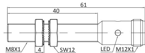
Fig. 2 Inductive sensor with M12 connector (flush)
