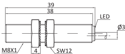
Fig. 1 Inductive sensor with cable (flush)
